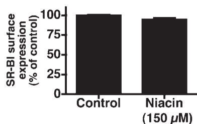
Fig. 2. Effects of niacin on scavenger receptor class B type I (SR-BI) activity in cells. Cells (IdIA[mSR-BI] and IdIA-7) were preincubated for 1 h at 37°C in medium containing the indicated concentrations of niacin. Subsequently, standard assays of SR-BI-mediated selective uptake of [ 3 H]cholesteryl oleyl ether (CE) from [ 3 H]CE-HDL (A), binding of 125 I-HDL (A), efflux of cellular unesterified [ 3 H]cholesterol to unlabeled HDL (B; average of two experiments), and the relative level of cell surface SR-BI determined by flow cytometry (C) were performed in the presence of the same concentration of niacin. The values were normalized so that 100% of control represents receptor-specific activity in IdIA[mSR-BI] cells in the presence of 0.5% DMSO without compounds. For selective uptake, binding, and efflux assays, 0% activity was defined as the activity determined in IdIA-7 cells, and for flow cytometry, the 0% of control values represent the background binding of KKB-1 to IdIA-7 cells. Values determined in the absence of niacin of [ 3 H]CE-HDL uptake, 125 I-HDL binding, and [ 3 H]cholesterol efflux were as follows: for IdIA[mSR-BI] cells, 6,766 ng protein (equivalent)/mg cell protein, 167 ng protein/mg, and 32% of the initial cellular [ 3 H]cholesterol level; for IdIA-7 cells: 968 ng/mg, 39 ng/mg, and 10%. Selective uptake was calculated as the difference between [ 3 H]CE-HDL uptake and 125 I-HDL binding.
